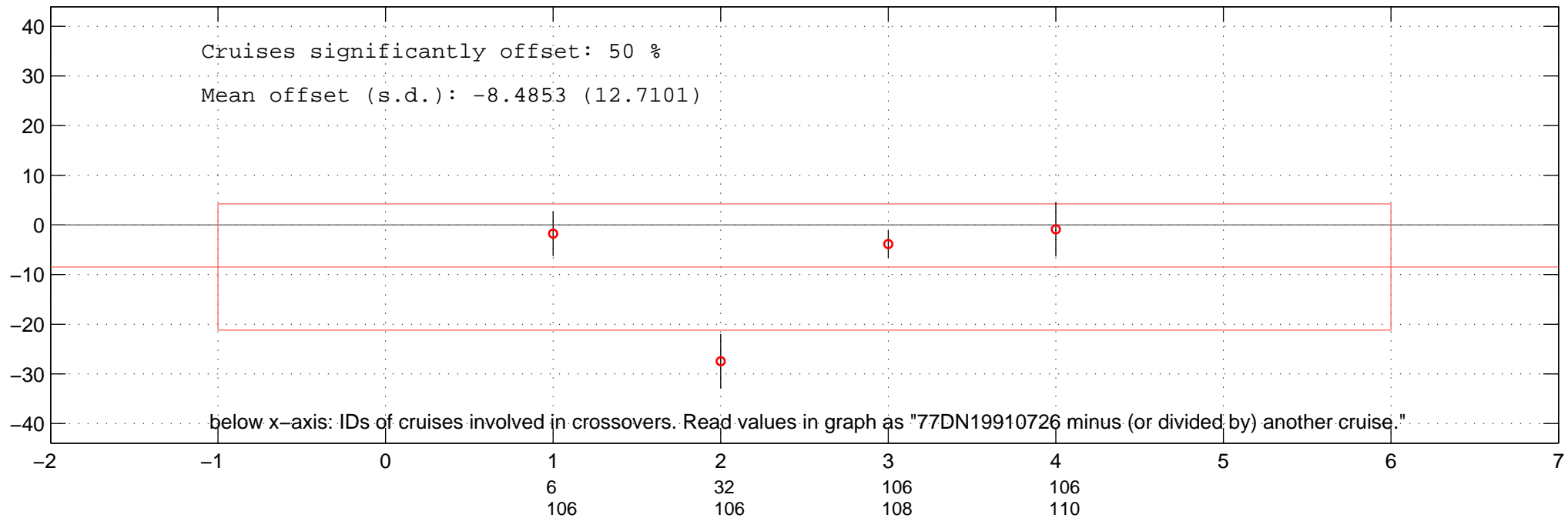
all additive offsets of ALK of 77DN19910726 in Favourite-space.
