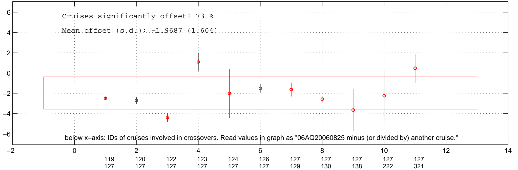
all multiplicative offsets of NO3 of 06AQ20060825 in Favourite-space.
