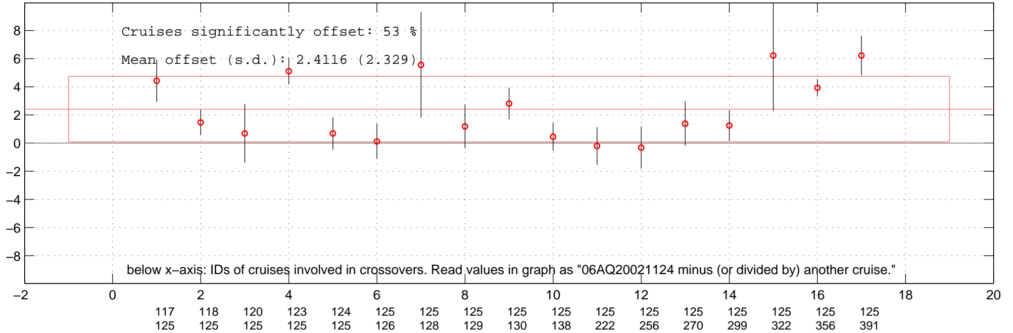
all multiplicative offsets of NO3 of 06AQ20021124 in Favourite-space.
