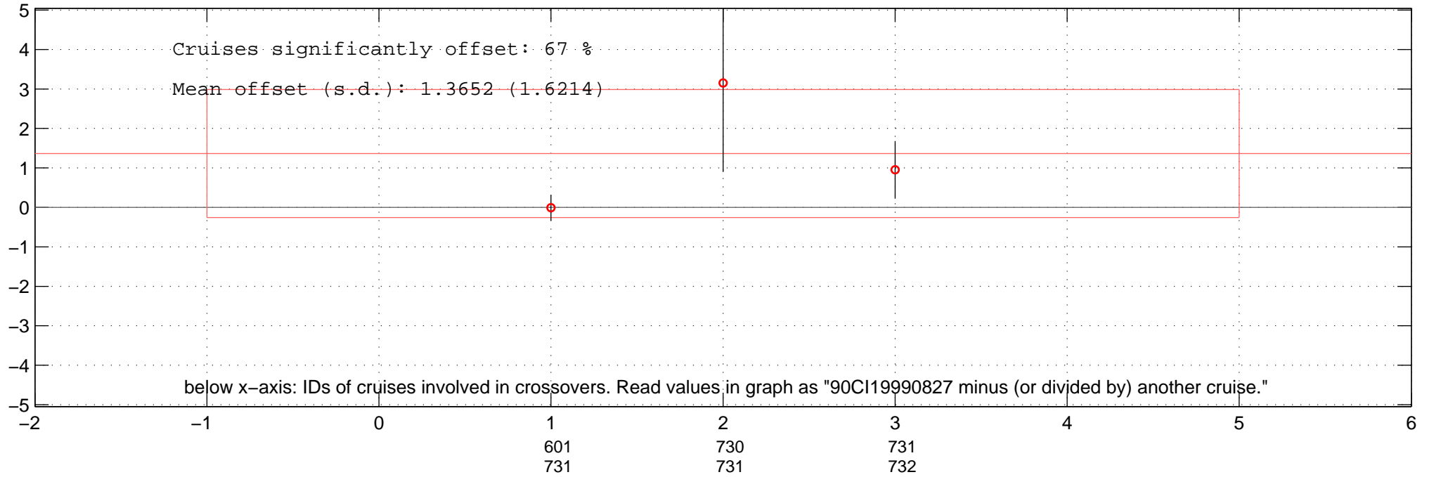
all multiplicative offsets of NO3 of 90CI19990827 in Favourite-space.
