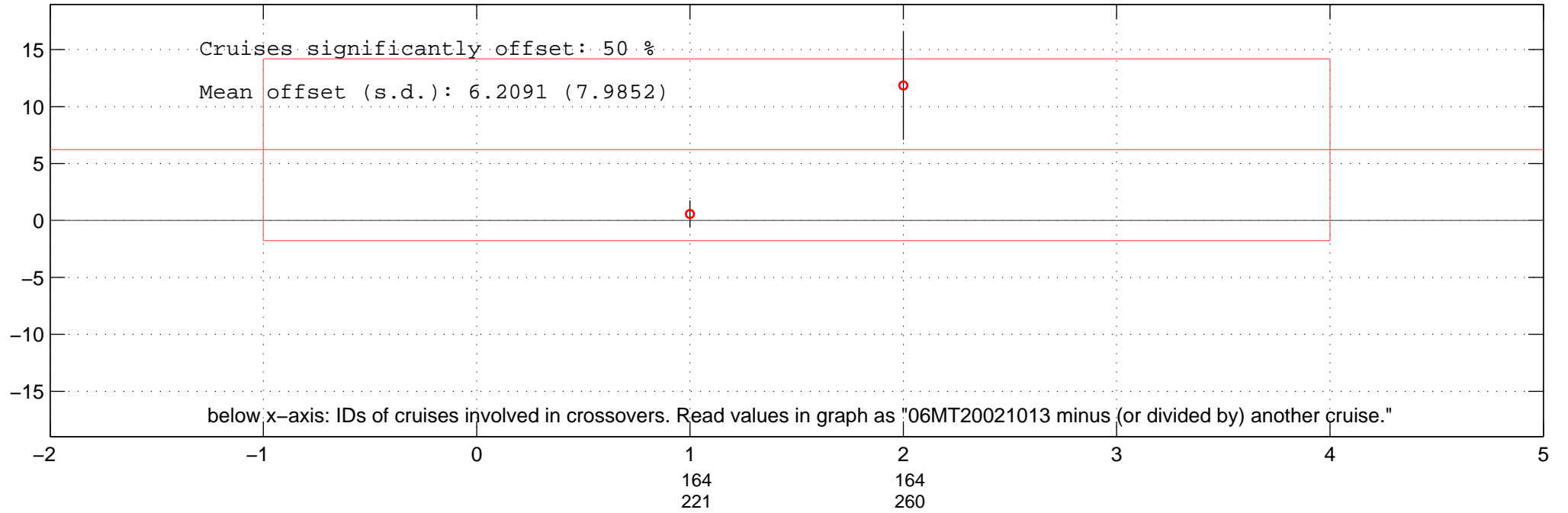
all multiplicative offsets of NO3 of 06MT20021013 in Favourite-space.
