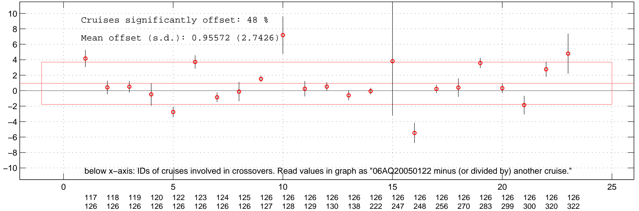
all multiplicative offsets of NO3 of 06AQ20050122 in Favourite-space.
