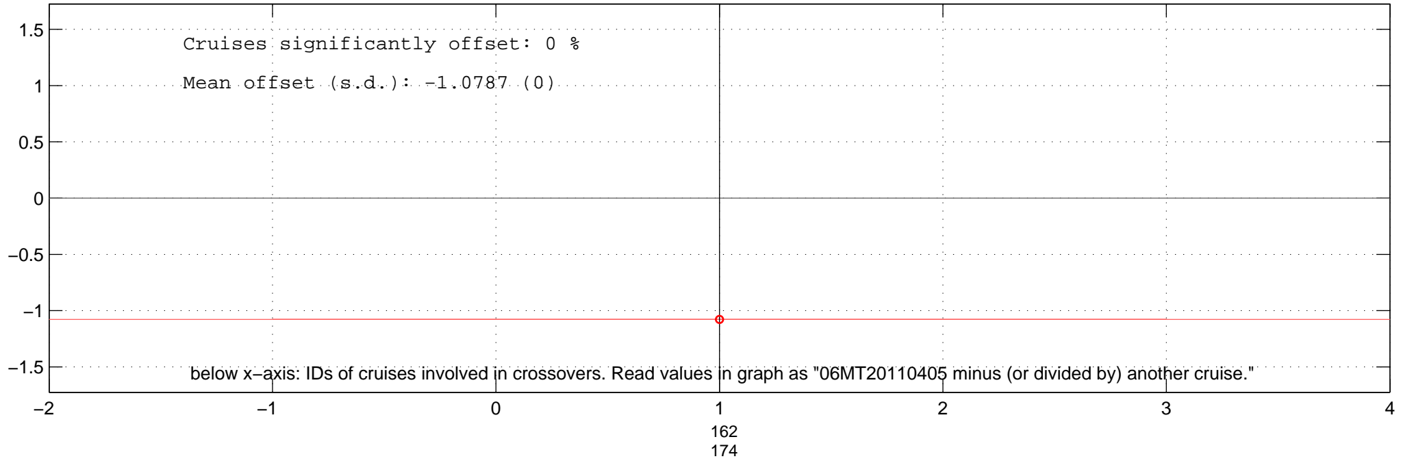
all multiplicative offsets of NO3 of 06MT20110405 in Favourite-space.
