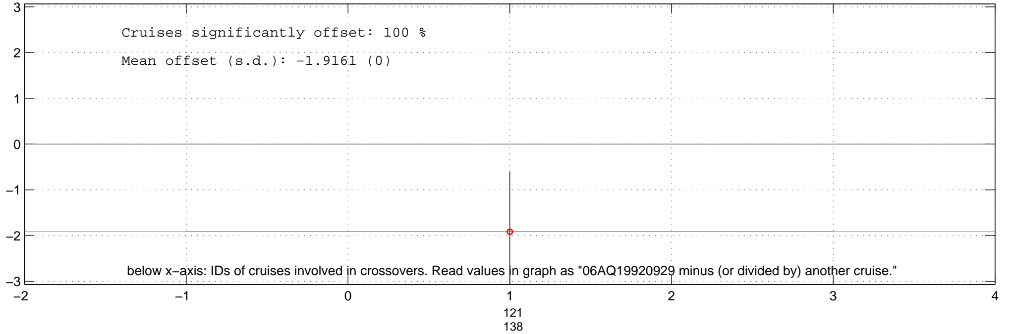
all multiplicative offsets of NO3 of 06AQ19920929 in Favourite-space.
