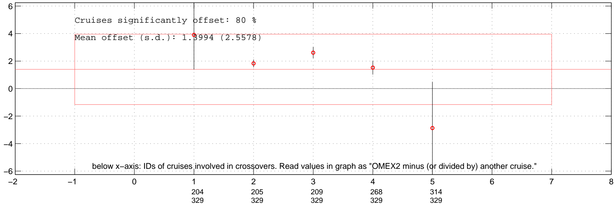
all multiplicative offsets of NO3 of OMEX2 in Favourite-space.
