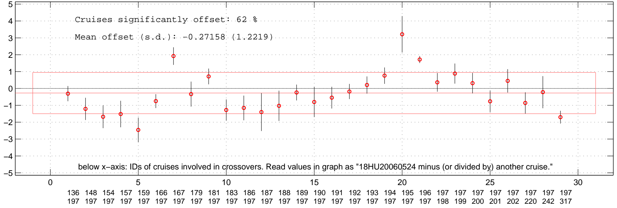
all multiplicative offsets of O2 of 18HU20060524 in Favourite-space.
