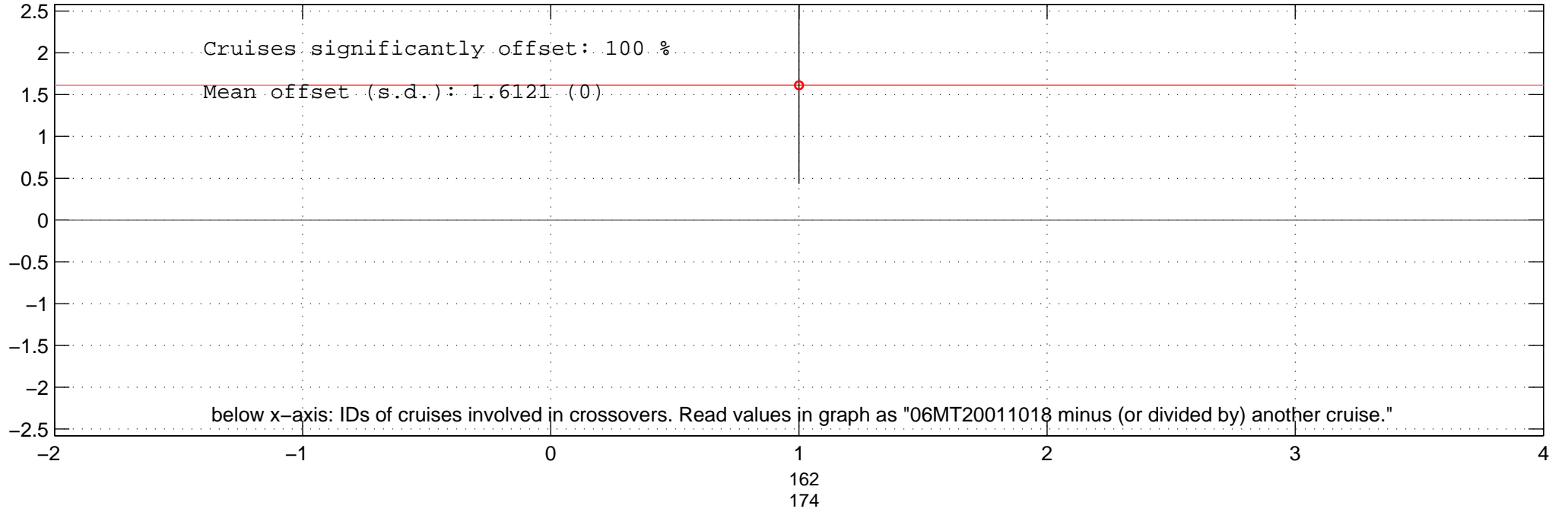
all multiplicative offsets of O2 of 06MT20011018 in Favourite-space.
