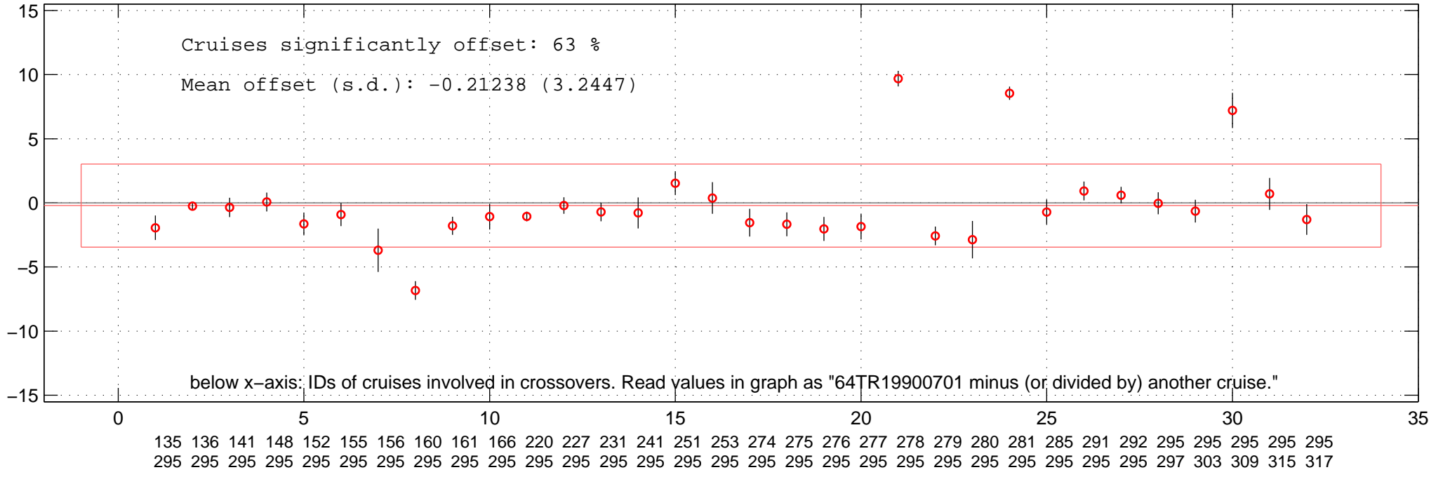
all multiplicative offsets of O2 of 64TR19900701 in Favourite-space.
