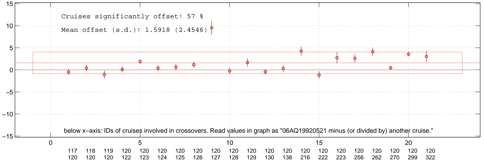
all multiplicative offsets of O2 of 06AQ19920521 in Favourite-space.
