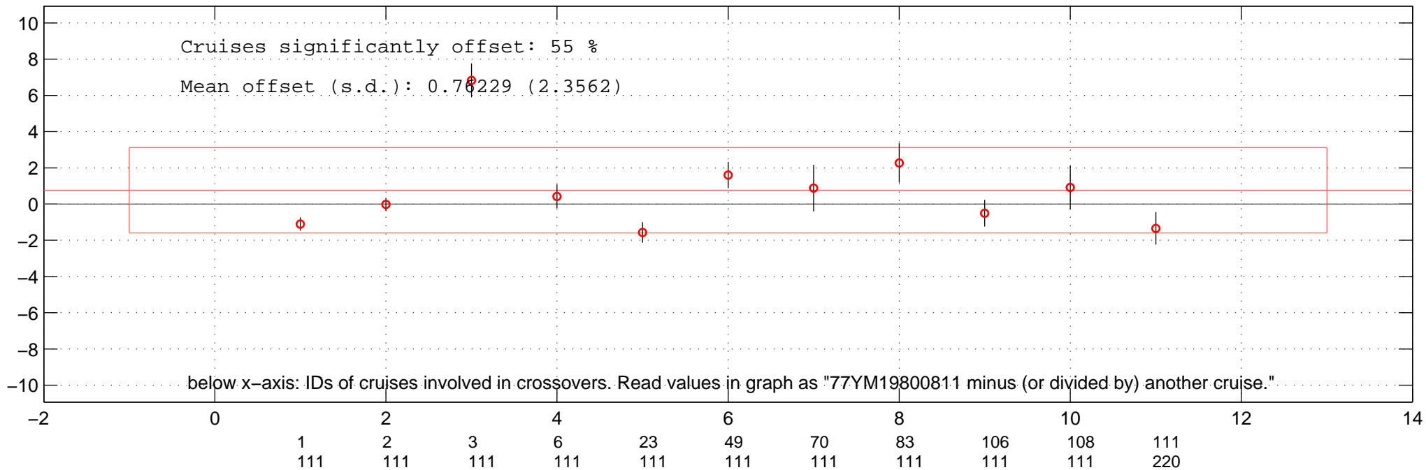
all multiplicative offsets of O2 of 77YM19800811 in Favourite-space.
