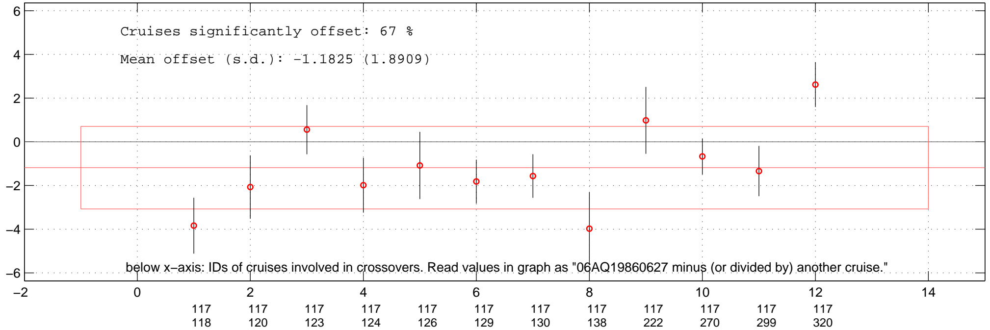
all multiplicative offsets of PO4 of 06AQ19860627 in Favourite-space.
