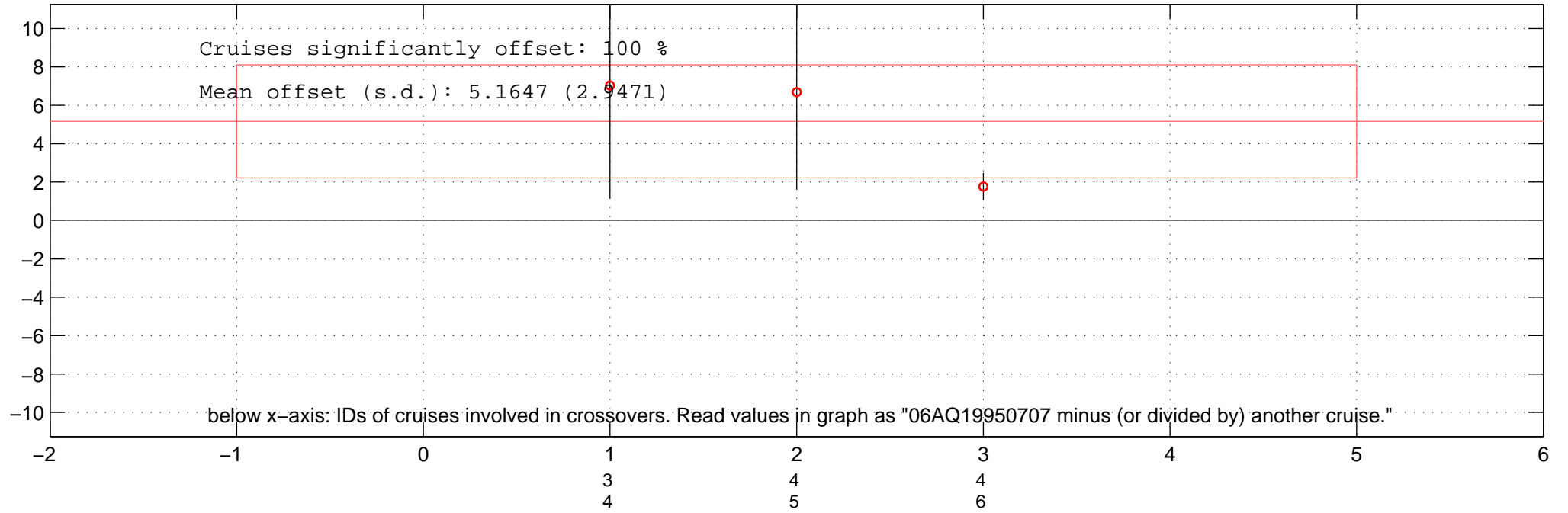
all multiplicative offsets of PO4 of 06AQ19950707 in Favourite-space.
