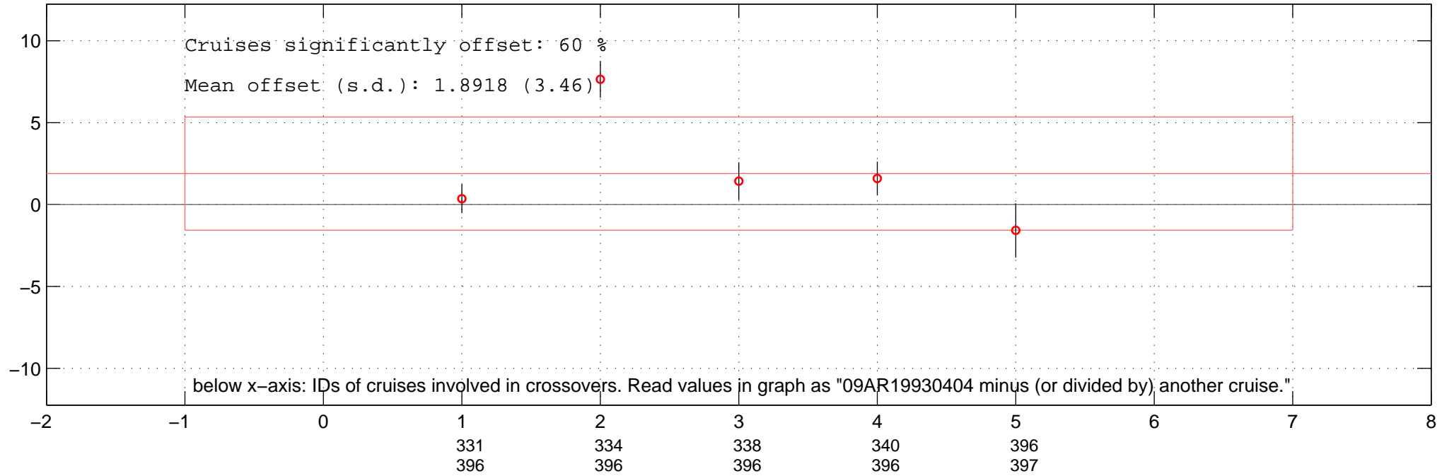
all multiplicative offsets of PO4 of 09AR19930404 in Favourite-space.
