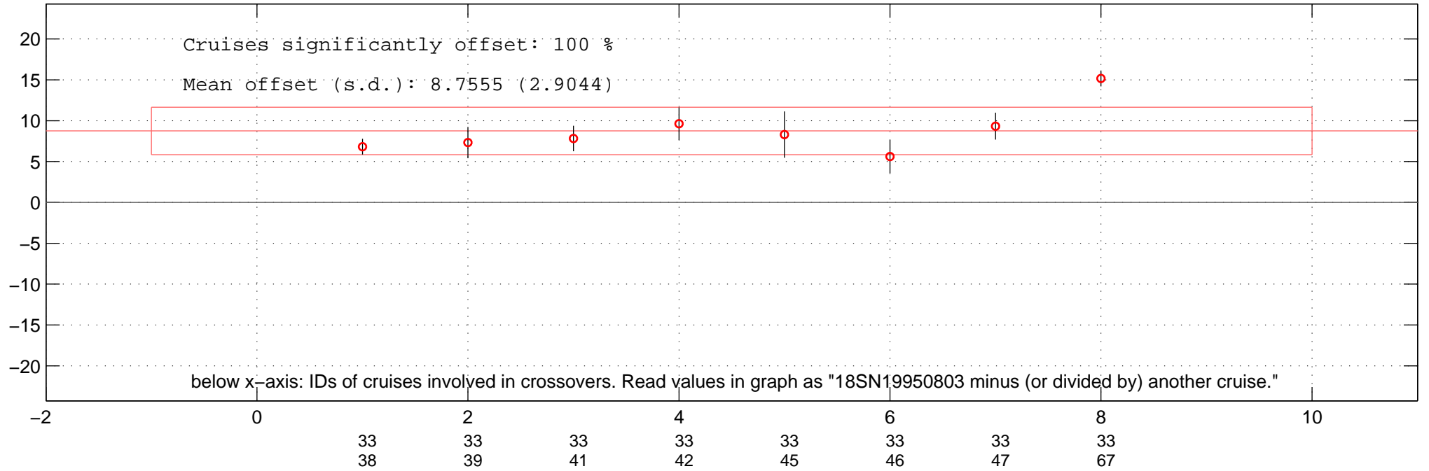
all multiplicative offsets of PO4 of 18SN19950803 in Favourite-space.
