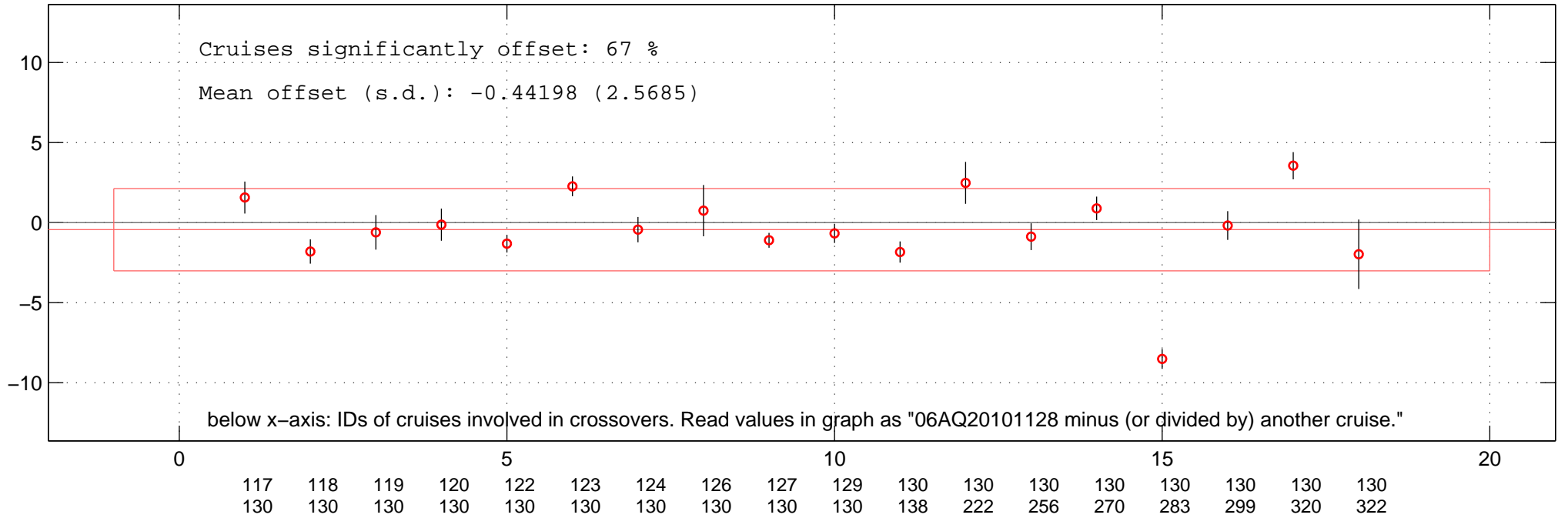
all multiplicative offsets of PO4 of 06AQ20101128 in Favourite-space.
