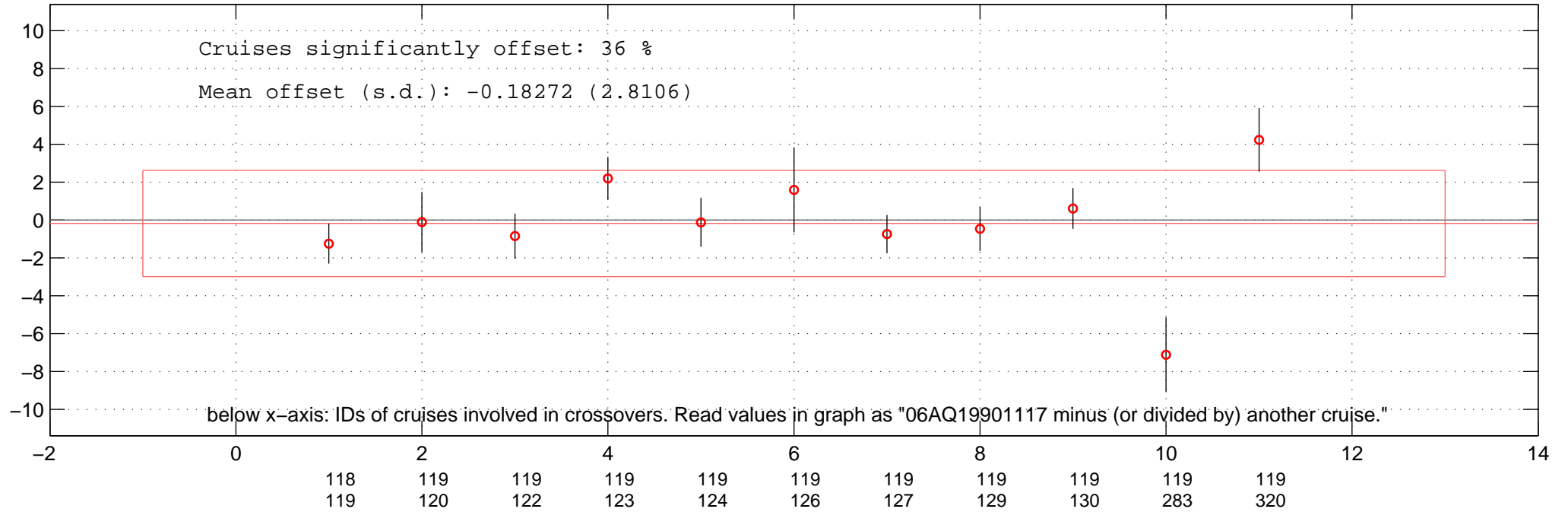
all multiplicative offsets of PO4 of 06AQ19901117 in Favourite-space.
