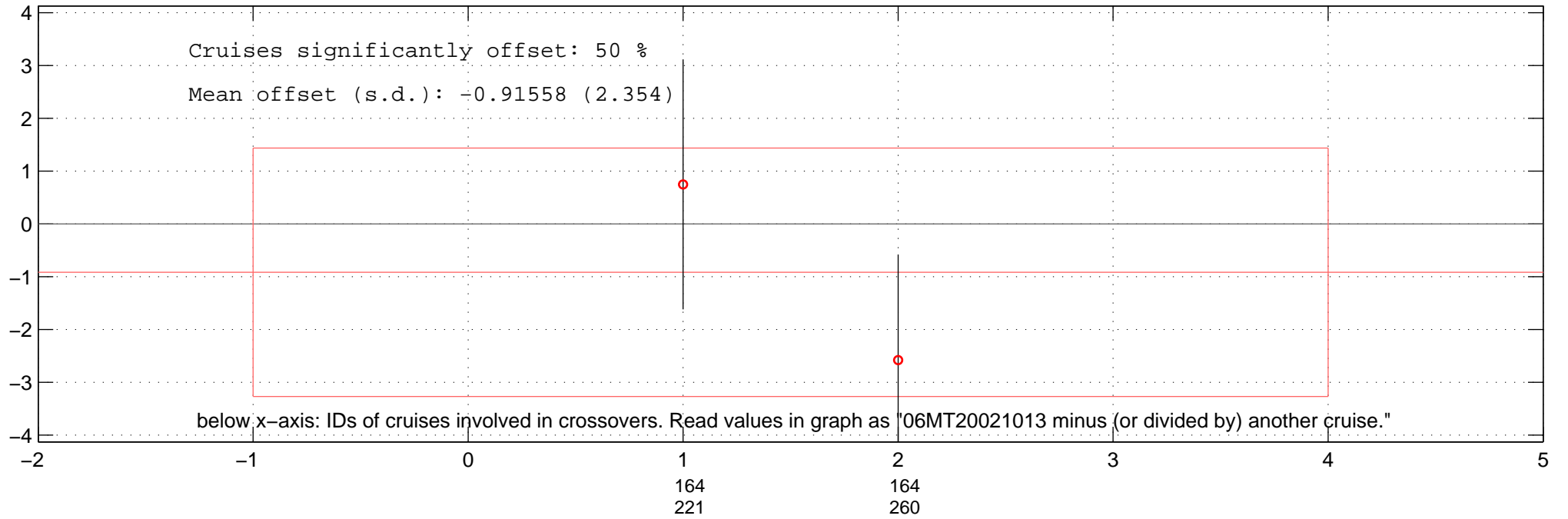
all multiplicative offsets of SIL of 06MT20021013 in Favourite-space.
