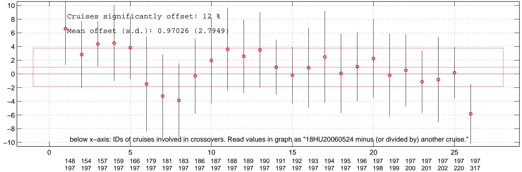
all multiplicative offsets of SIL of 18HU20060524 in Favourite-space.
