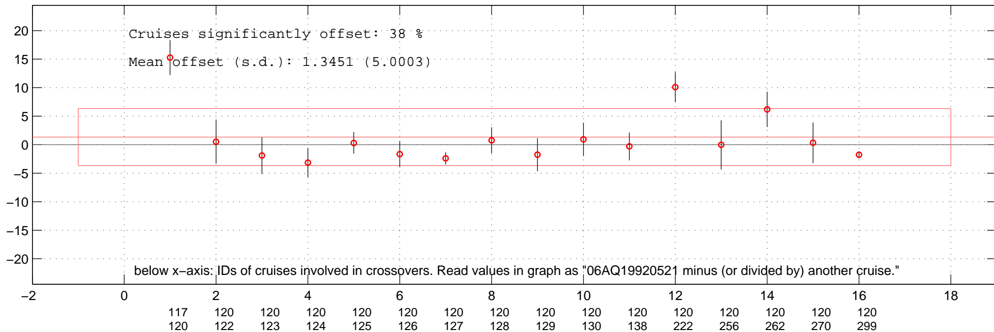
all additive offsets of DIC of 06AQ19920521 in Favourite-space.
