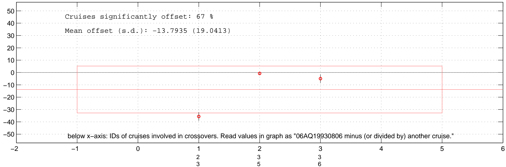
all additive offsets of DIC of 06AQ19930806 in Favourite-space.
