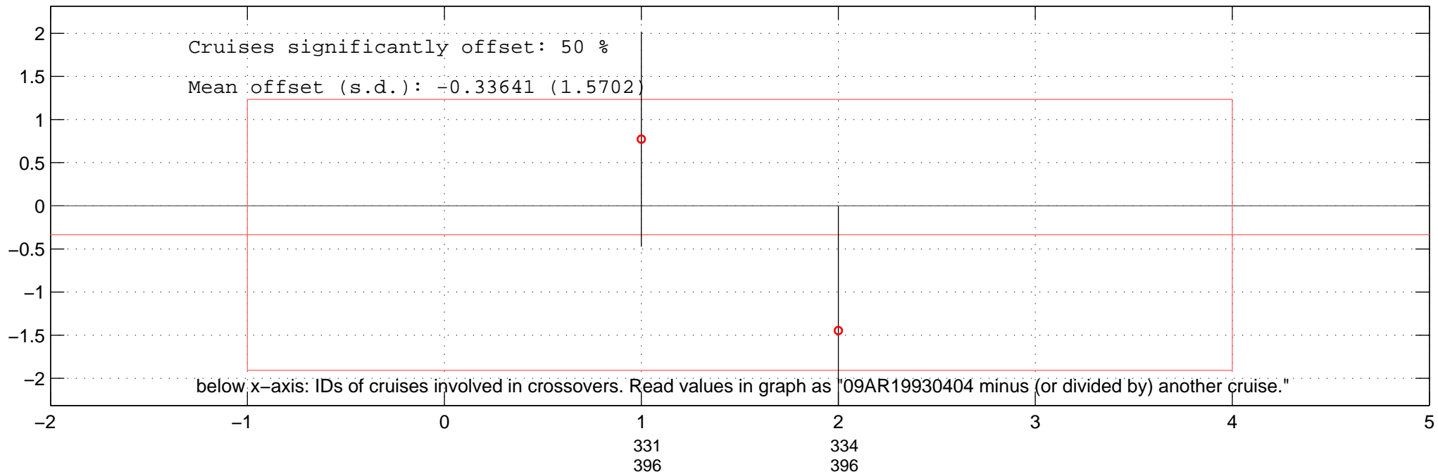
all additive offsets of DIC of 09AR19930404 in Favourite-space.
