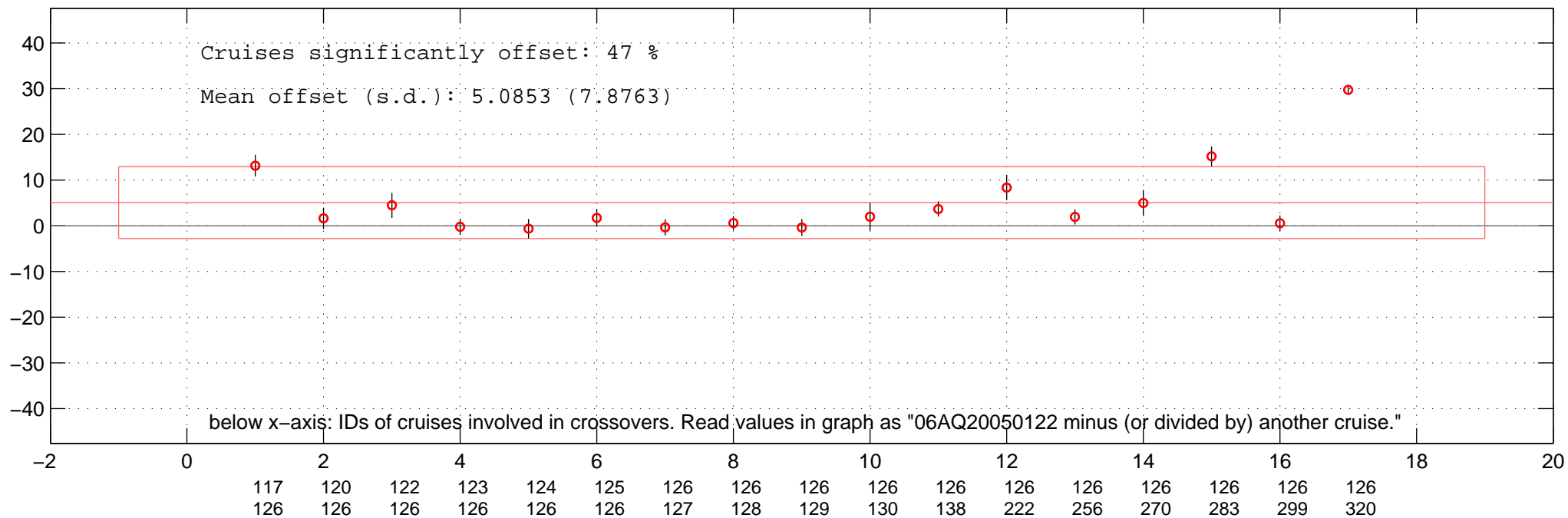
all additive offsets of DIC of 06AQ20050122 in Favourite-space.
