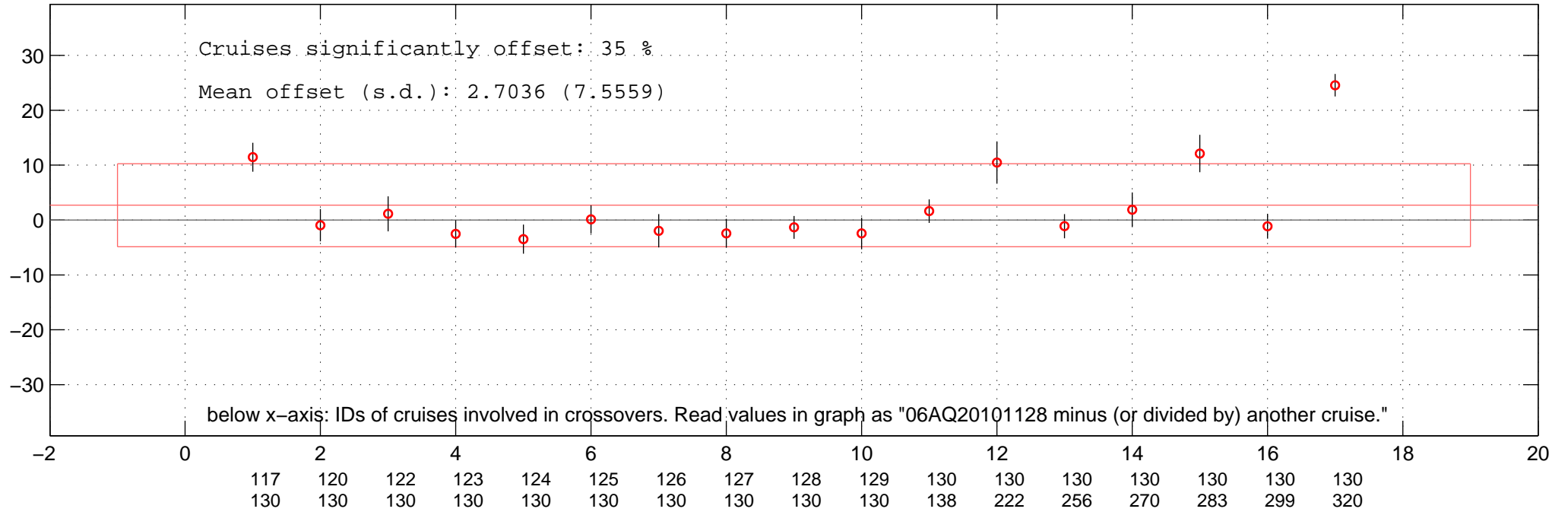
all additive offsets of DIC of 06AQ20101128 in Favourite-space.
