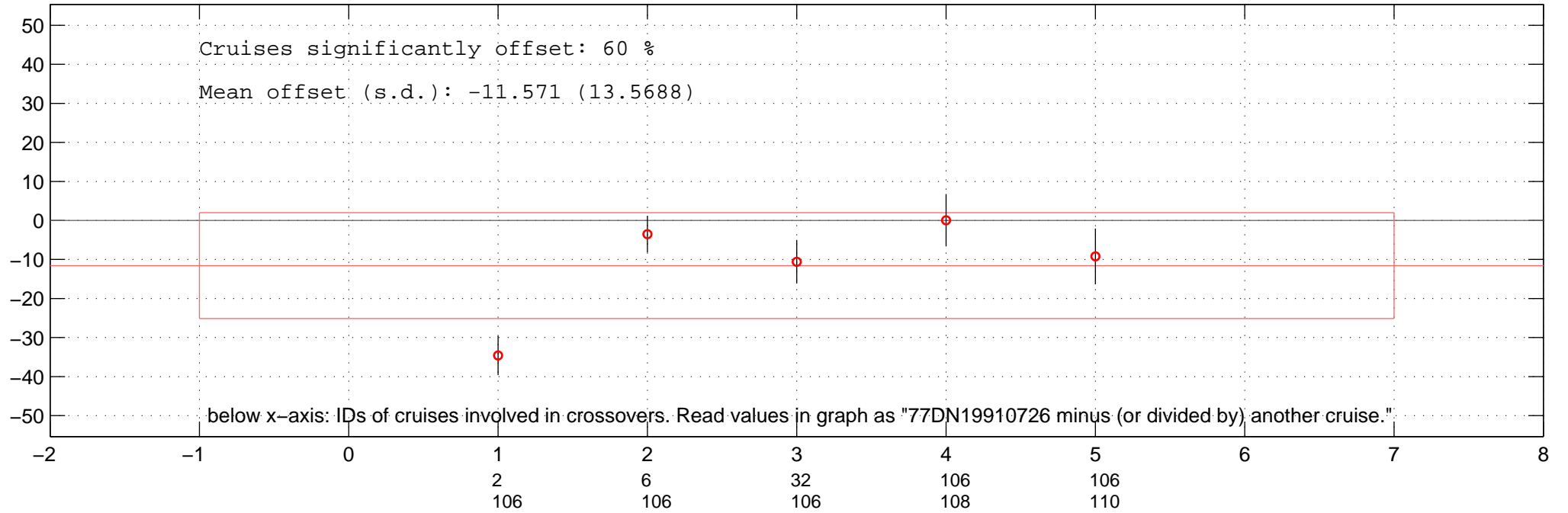
all additive offsets of DIC of 77DN19910726 in Favourite-space.
