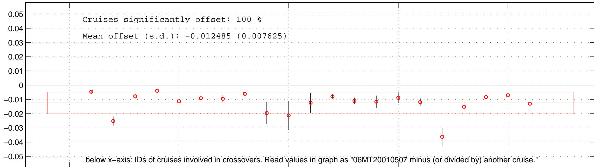
all additive offsets of SAL of 06MT20010507 in Favourite-space.
