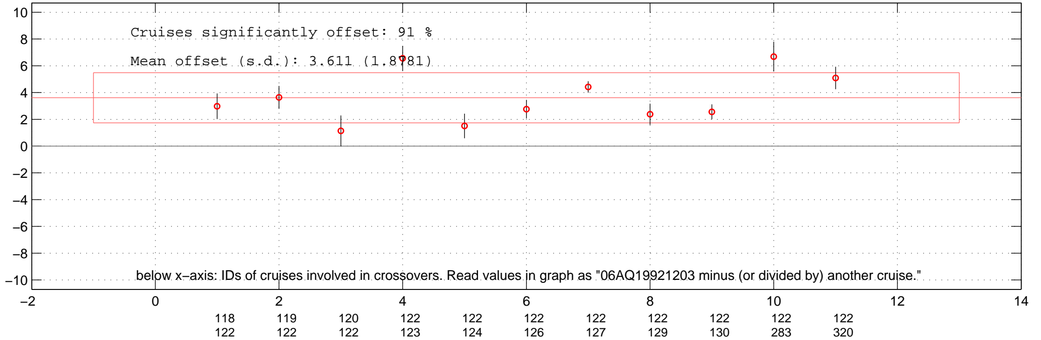
all multiplicative offsets of NO3 of 06AQ19921203 in Favourite-space.
