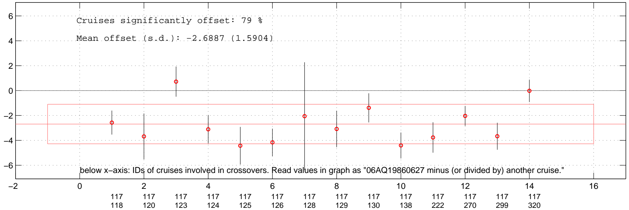
all multiplicative offsets of NO3 of 06AQ19860627 in Favourite-space.
