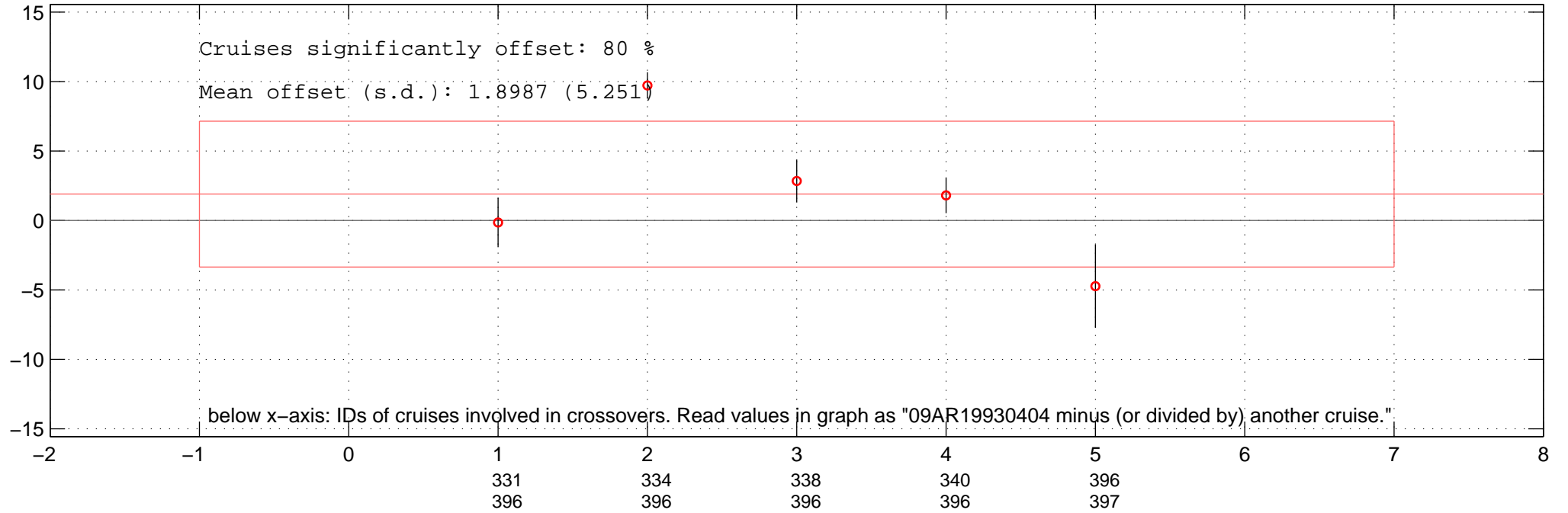
all multiplicative offsets of NO3 of 09AR19930404 in Favourite-space.
