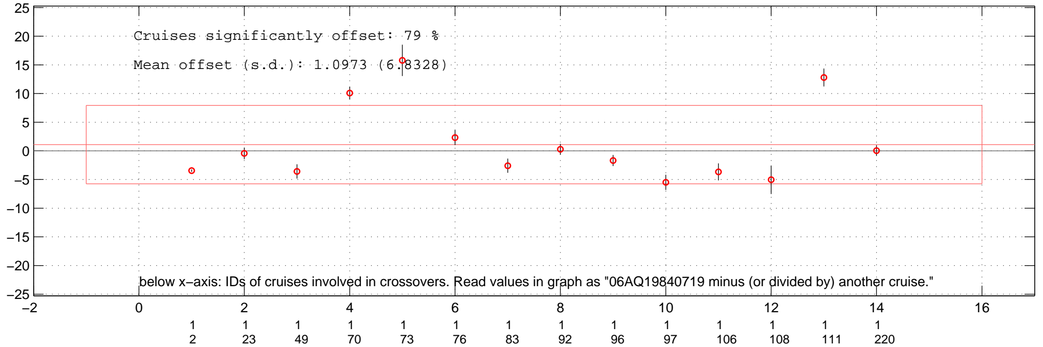
all multiplicative offsets of NO3 of 06AQ19840719 in Favourite-space.
