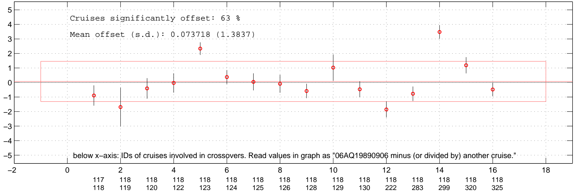
all multiplicative offsets of O2 of 06AQ19890906 in Favourite-space.
