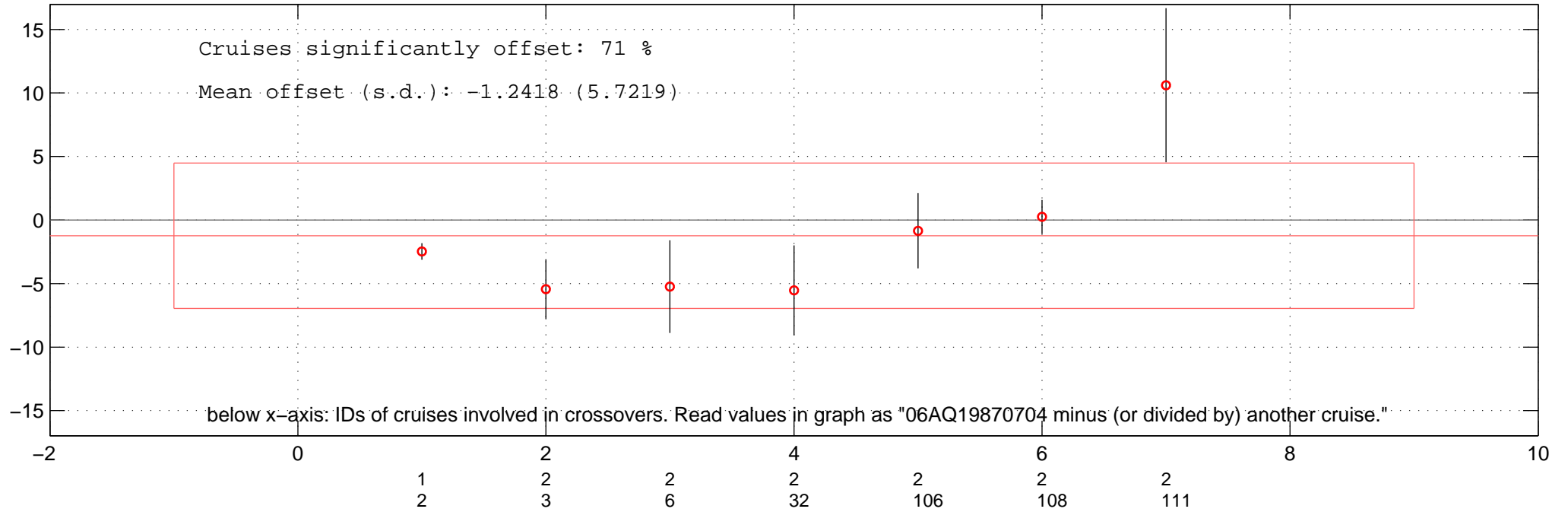
all multiplicative offsets of PO4 of 06AQ19870704 in Favourite-space.
