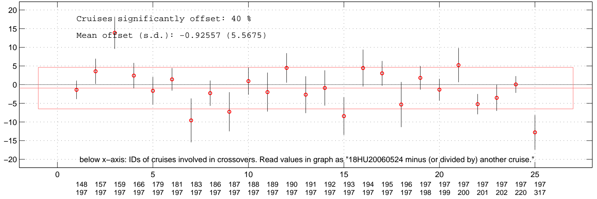
all multiplicative offsets of PO4 of 18HU20060524 in Favourite-space.
