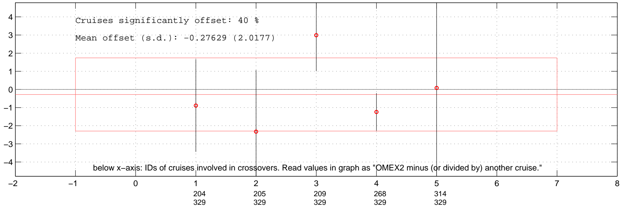
all multiplicative offsets of PO4 of OMEX2 in Favourite-space.
