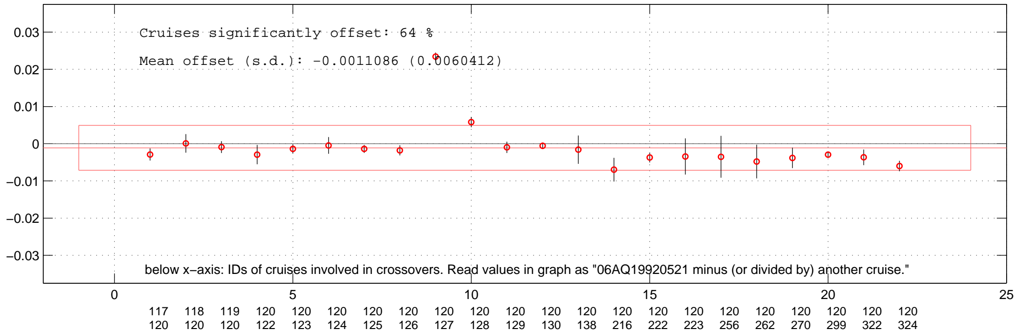
all additive offsets of SAL of 06AQ19920521 in Favourite-space.
