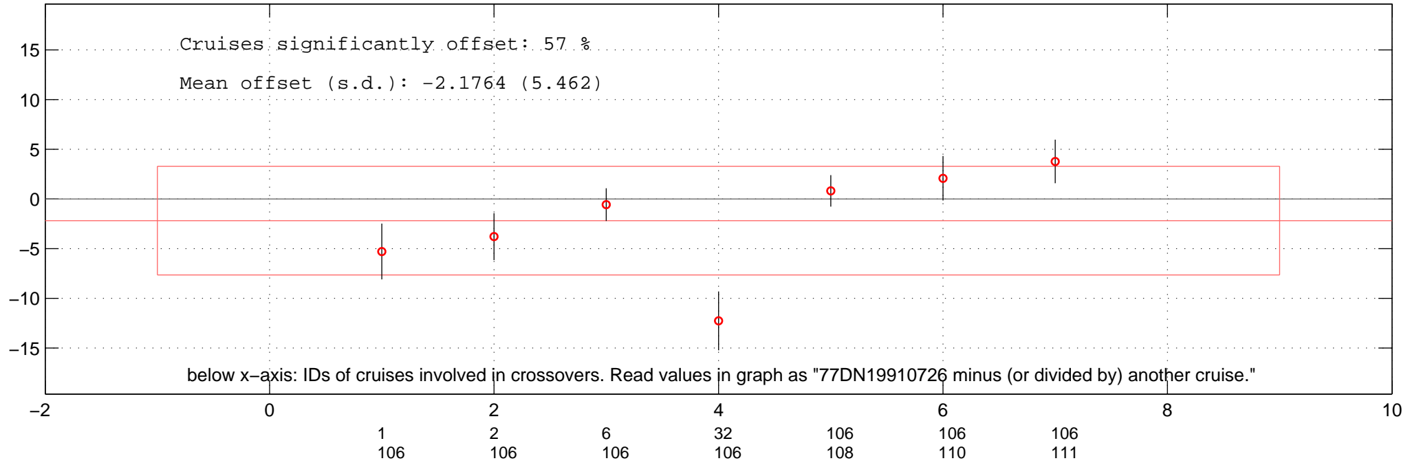
all multiplicative offsets of SIL of 77DN19910726 in Favourite-space.
