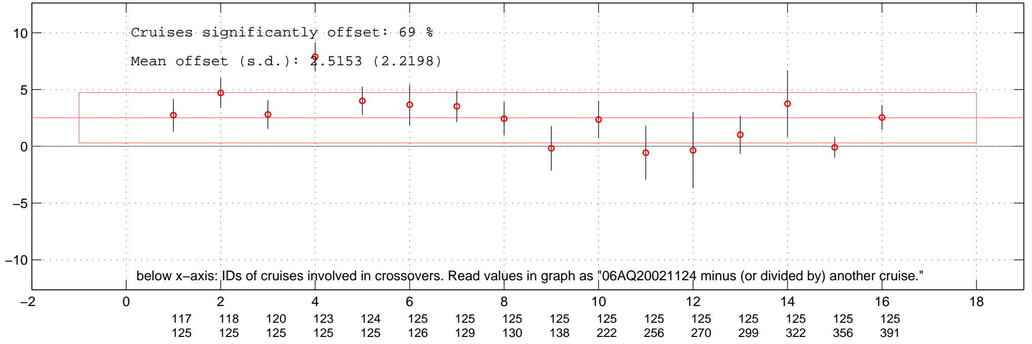
all multiplicative offsets of SIL of 06AQ20021124 in Favourite-space.
