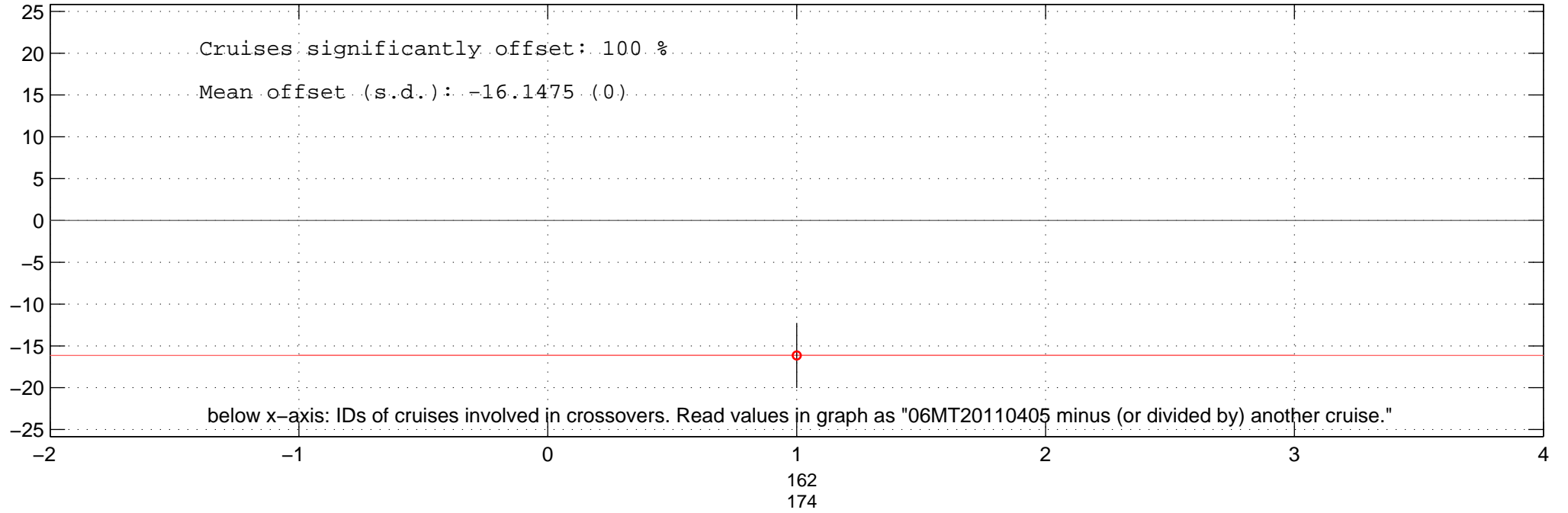
all multiplicative offsets of SIL of 06MT20110405 in Favourite-space.
