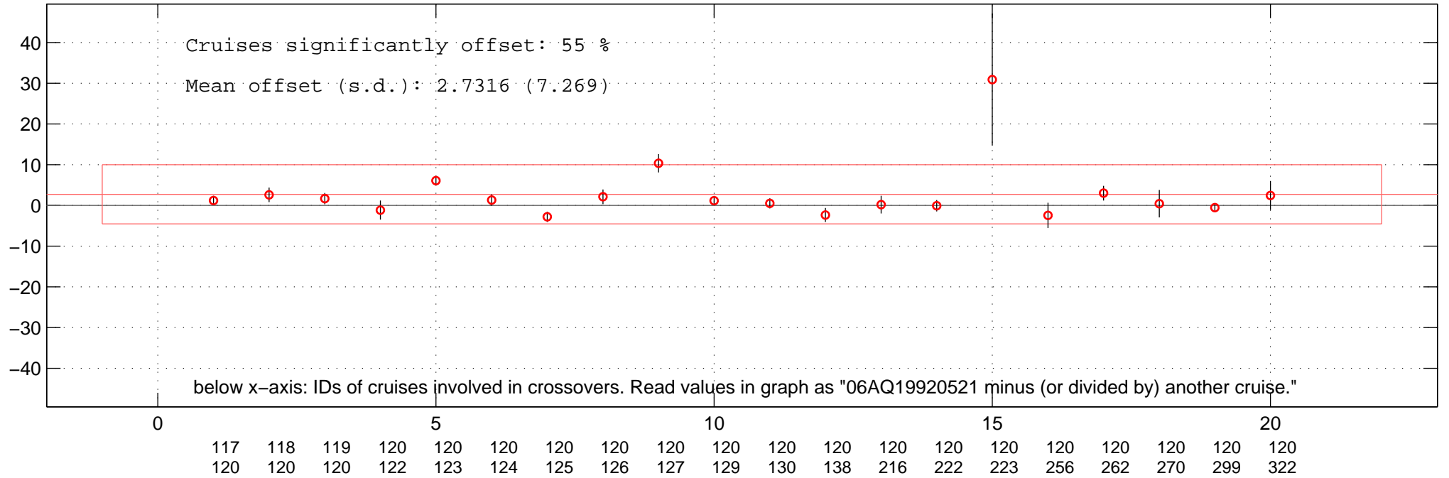
all multiplicative offsets of SIL of 06AQ19920521 in Favourite-space.
