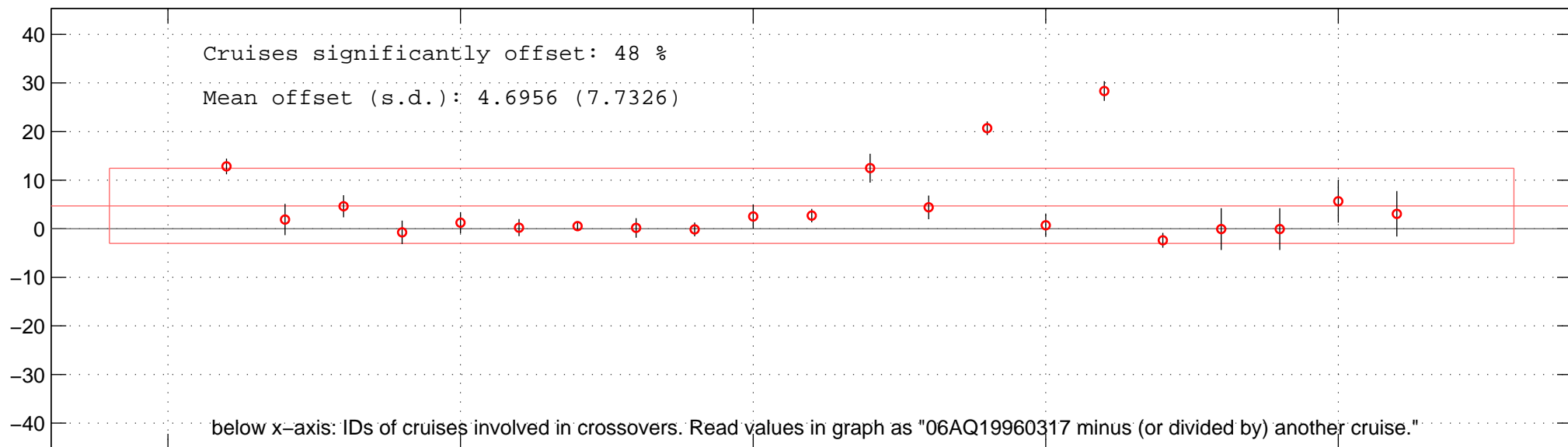
all additive offsets of DIC of 06AQ19960317 in Favourite-space.
