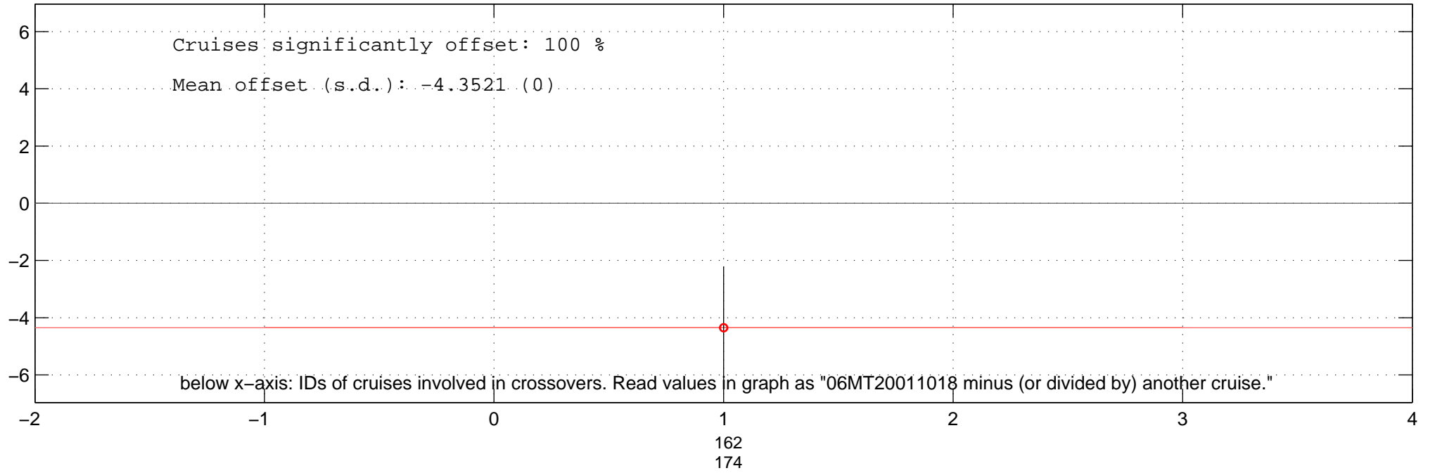
all additive offsets of DIC of 06MT20011018 in Favourite-space.
