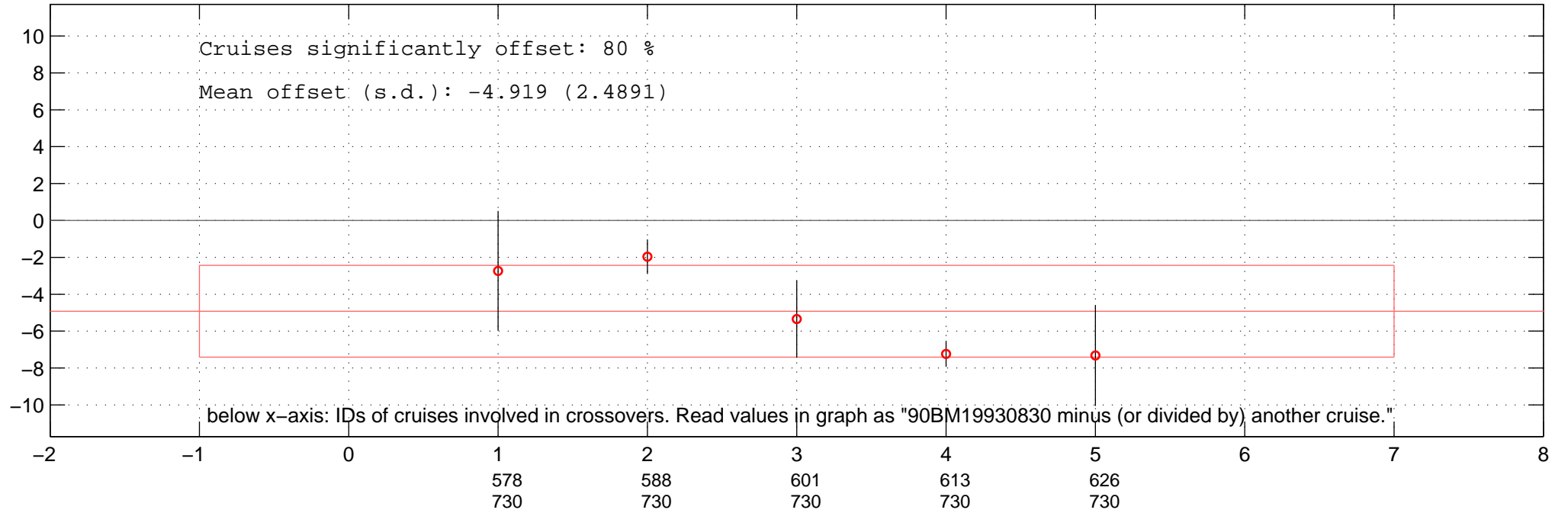
all additive offsets of DIC of 90BM19930830 in Favourite-space.
