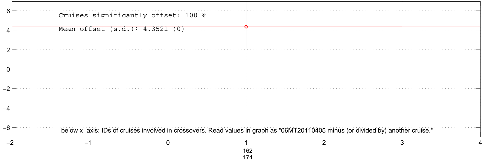
all additive offsets of DIC of 06MT20110405 in Favourite-space.
